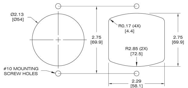
Round cutout for front or rear mount
